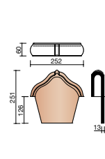
M000 1340 Fronton standard
