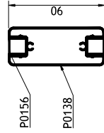
Section Vertical
