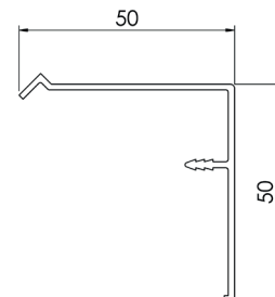
Angle 50 mm BRA3
