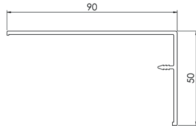
Angle 90 mm BRC3
