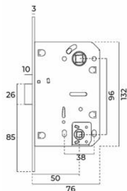
SERRURE A CONdamnATION / WC Ref.IN.20.836.50
