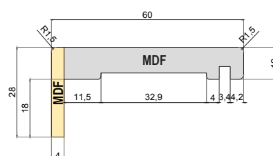
Couvre joints section. 60x28mm Hauteur 2131mm
