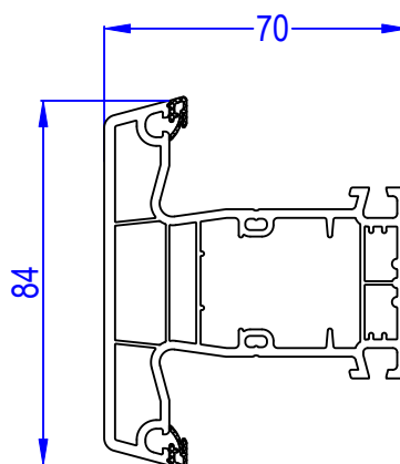
Traverse 84 mm 140441
