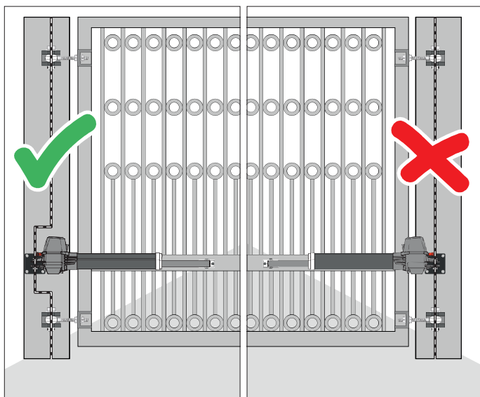
III. 1 Point de rotation correct III. 2 Point de rotation incorrect
